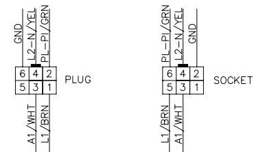
CONECTOR 230V MONITOR 6pin
